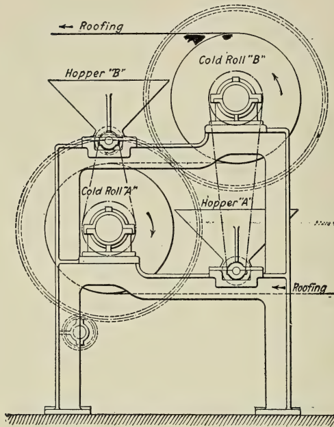
FIG. 130.—Device for Applying Mineral Particles to the Surface of Prepared Roofing
